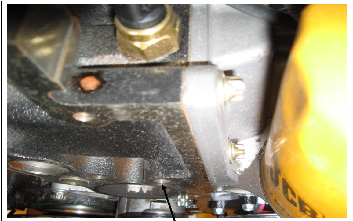
Mount the back side idler pulley in this M10 threaded hole.
